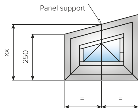
Slanted window
