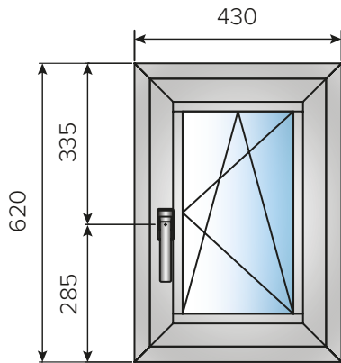
Tilt-and-turn window
